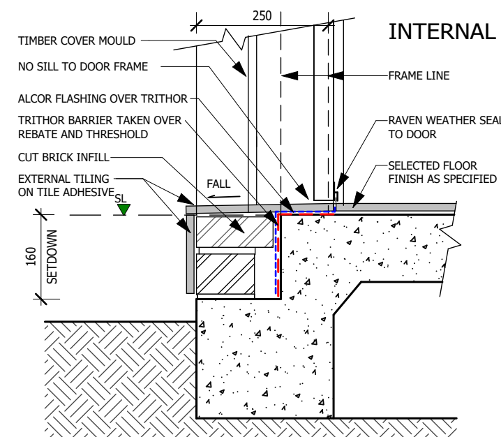
4 LAUNDRY TIMBER DOOR SCALE: 1 : 10
