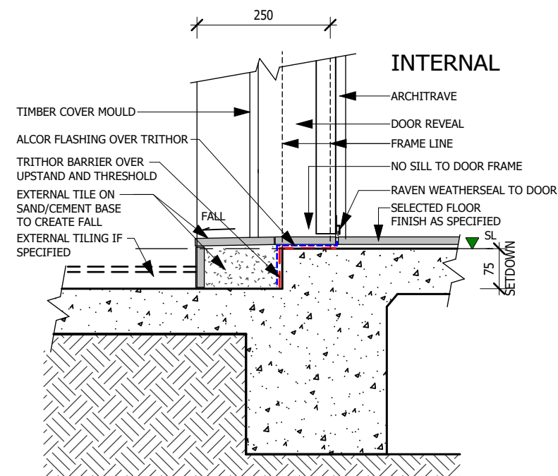
2 BRICK VENEER PORCH ENTRY DOOR SCALE: 1 : 10
