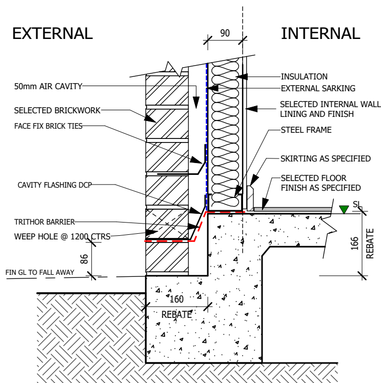
1 BRICK VENEER REBATE DETAIL SCALE: 1 : 10
