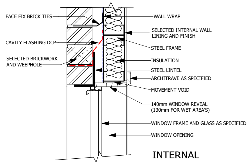
1 WINDOW HEAD - BRICK VENEER SCALE: 1 : 10
