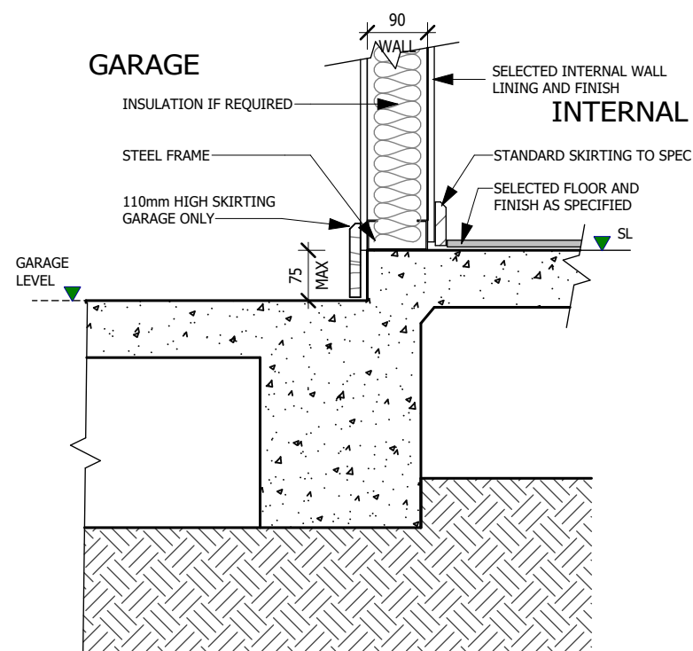
4 INTERNA GARAGE STEP - 75MM STEP ONLY1 SCALE: 1 : 10
