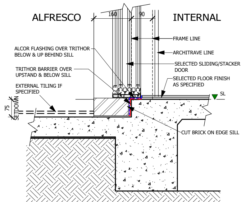
3 ALFRESCO DOOR - BRICK VENEER SCALE: 1 : 10
