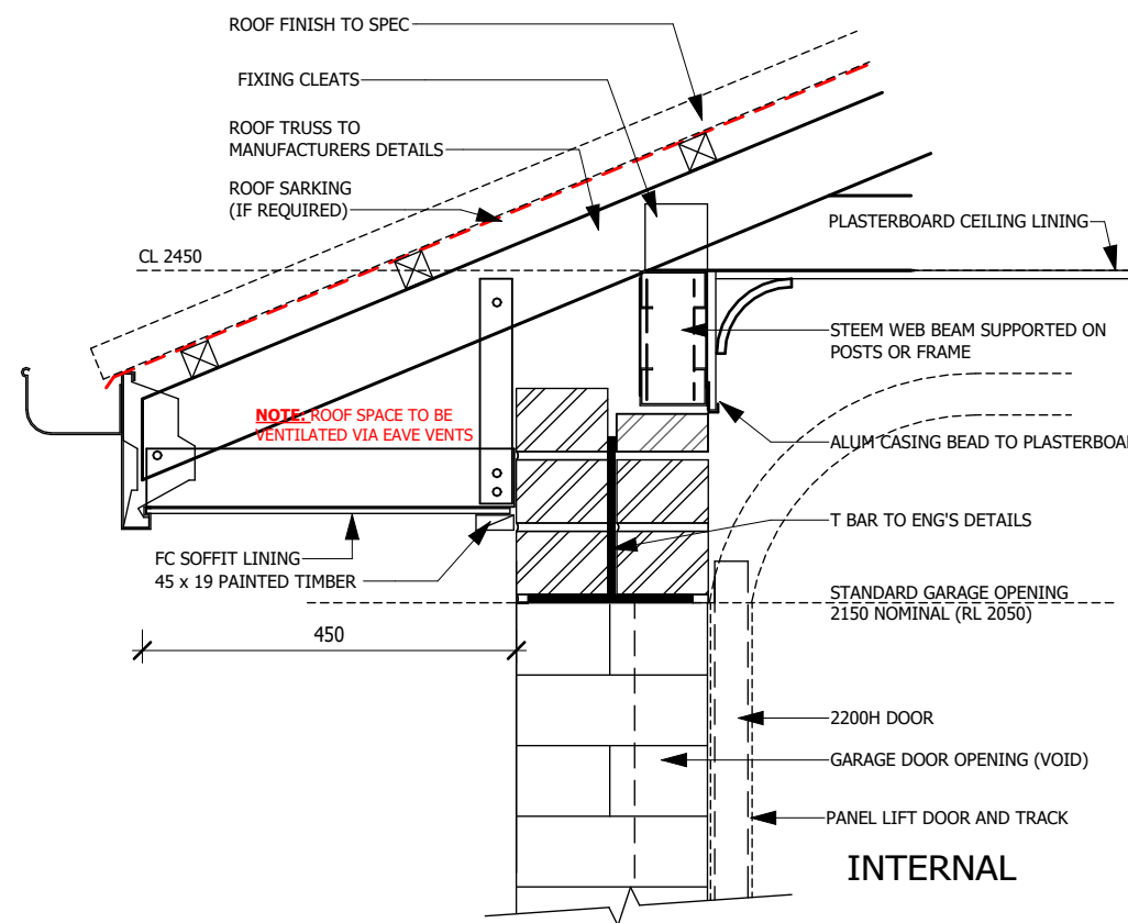
4 GARAGE DOOR HEAD DETAIL EAVES ABOVE SCALE: 1 : 10
