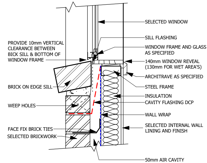
2 WINDOW SILL - BRICK VENEER SCALE: 1 : 10
