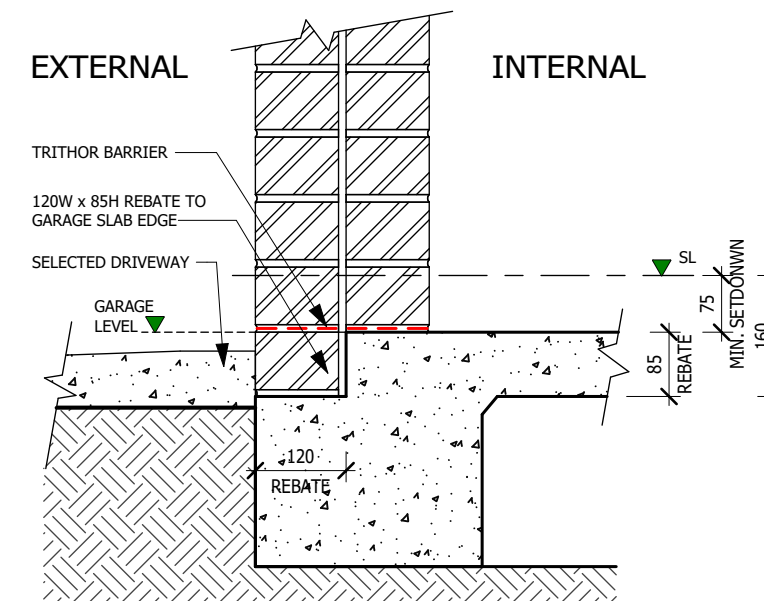
2 GARAGE REBATE (FRONT SIDE OF DOOR) SCALE: 1 : 10
