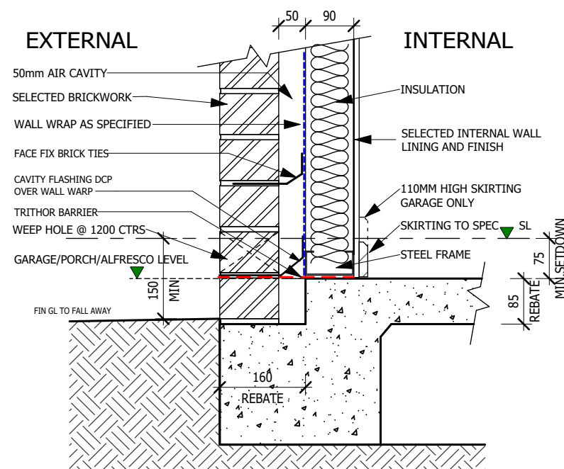
1 GARAGE REBATE (SIDE) & PORCH/ALFRESCO SCALE: 1 : 10
